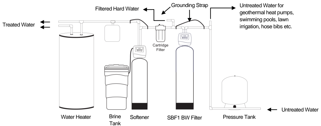
FIGURE 1: Typical Installation
