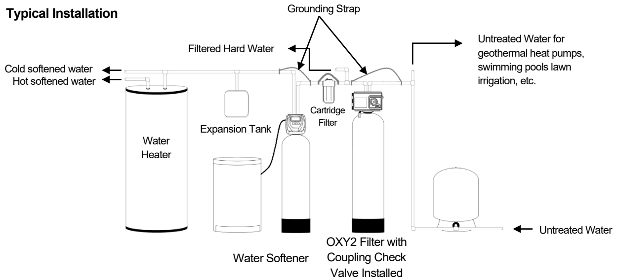
FIGURE 1: Typical Installation
